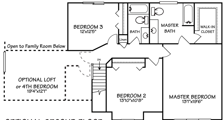
OPTIONAL SECOND FLOOR 3 BEDROOM PLAN
