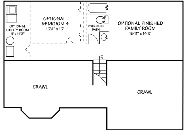
LOWER LEVEL FLOOR PLAN ON CRAWL
