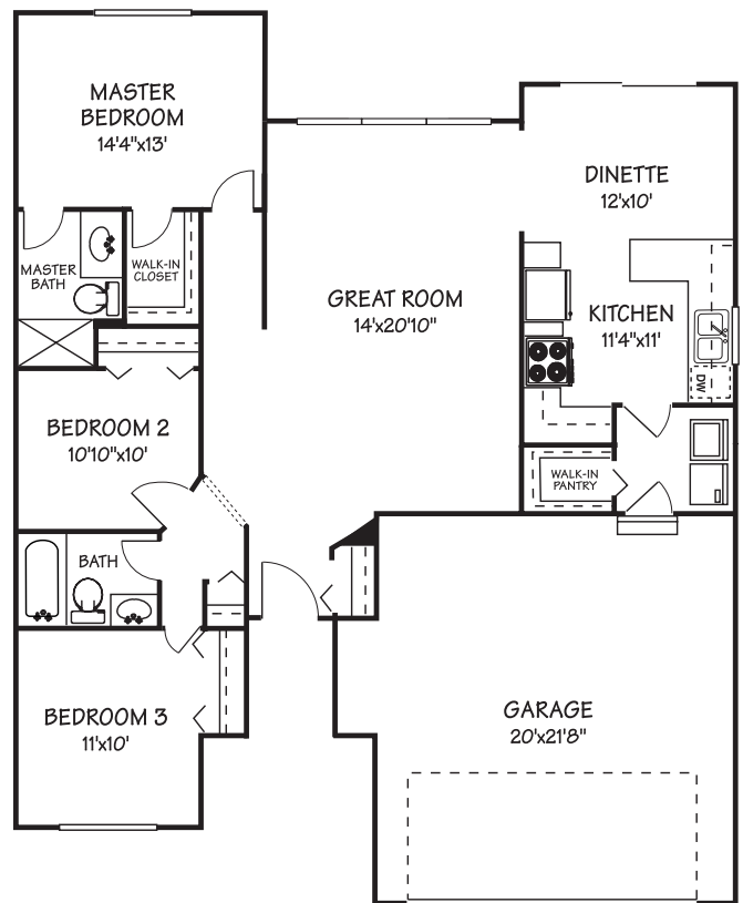
OPTIONAL THREE BEDROOM FLOOR PLAN
